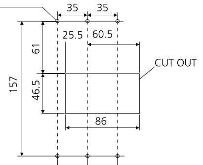
Mounting & Door Cut-out Details
